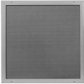
RA-P 3/16" holes at 1/4" on center 50% free area
